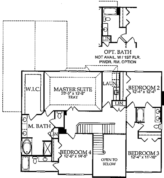
Second Floor 8'-0" CEILING
