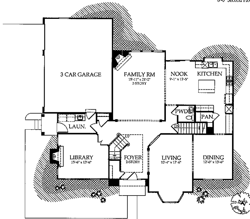
First Floor 9'-0" First Floor Ceiling
